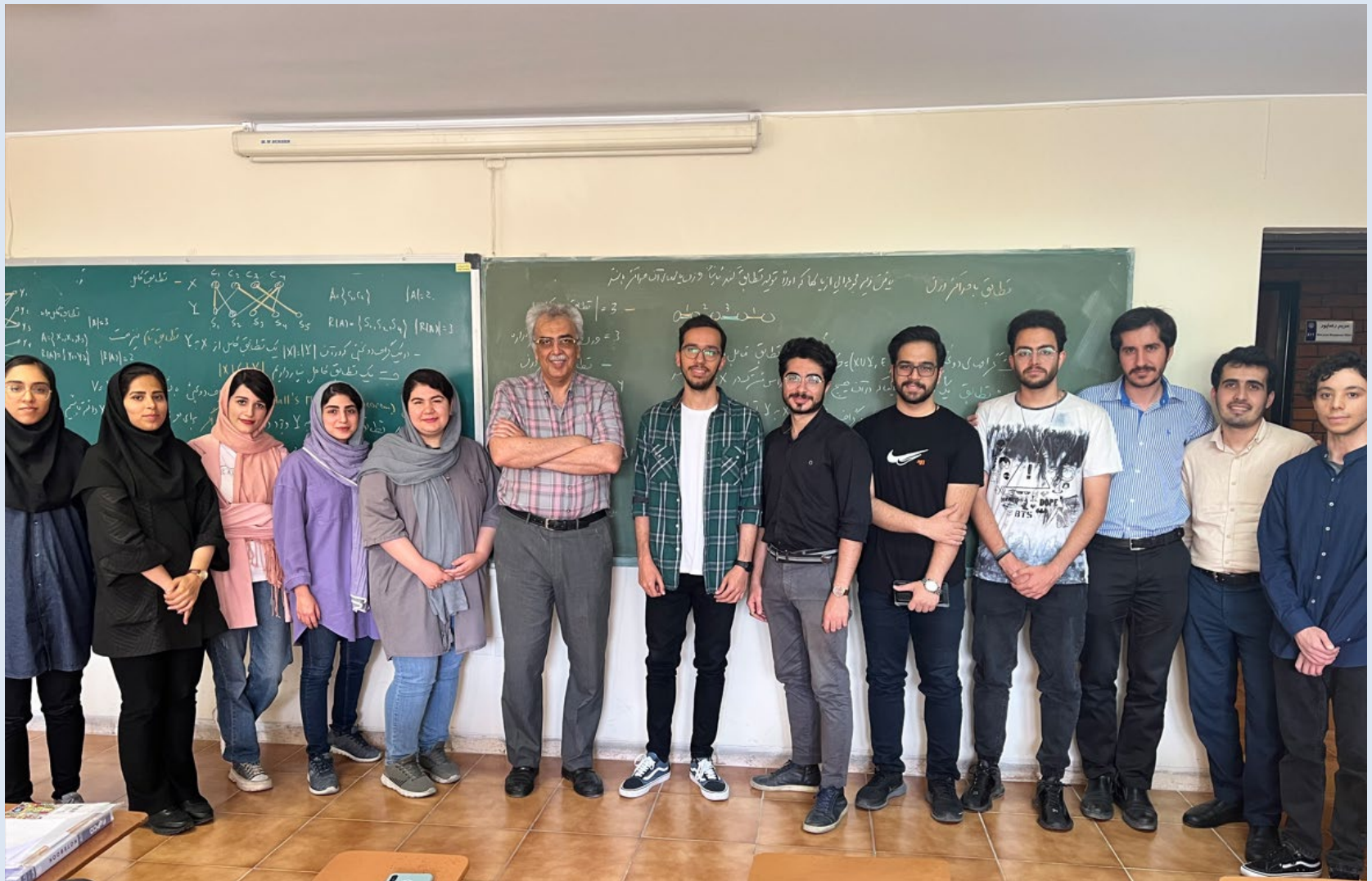
Graph Theory Class-2023
